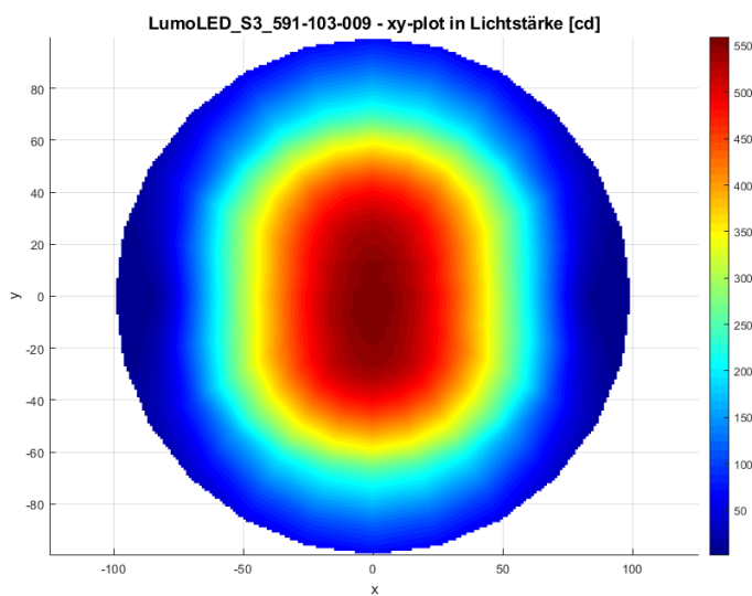
Distribution of the luminous intensity based on LumoLED S3 | Item no. 591-103-009
