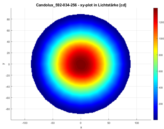
Distribution of the luminous intensity based on Candolux/034256 | Item no. 592-034-256
