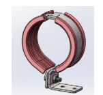
ITEM NO. 599-001-022 Fixing clamp Ø70 mm, stainless steel A4, angle plug, wall clearance 70 mm
